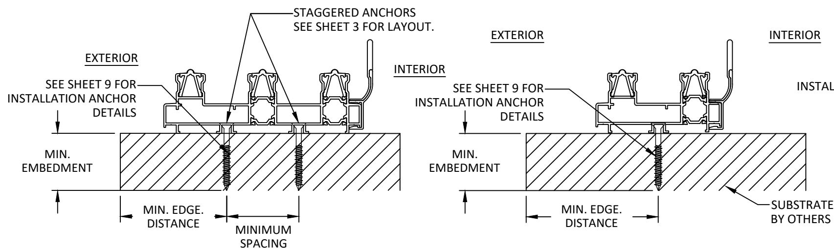
E 8 ANCHOR DETAIL THROUGH FRAME INSTALLATION (SILL) 3 TRACKS SHOWN, 4 TRACKS SIMILAR
