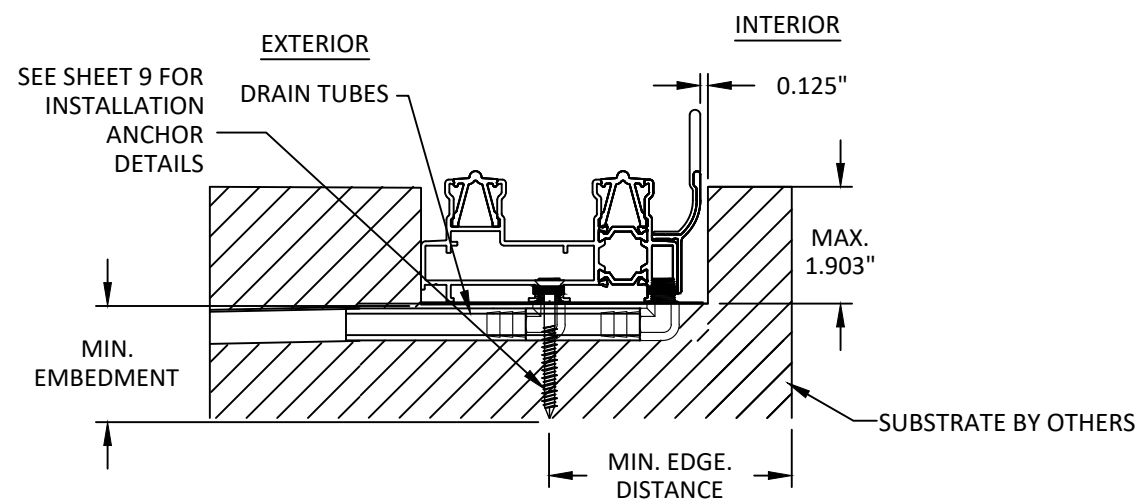
D 8 ANCHOR DETAIL THROUGH FRAME INSTALLATION (SILL) OPTIONAL SUNKEN 2-TRACK INSTALLATION
